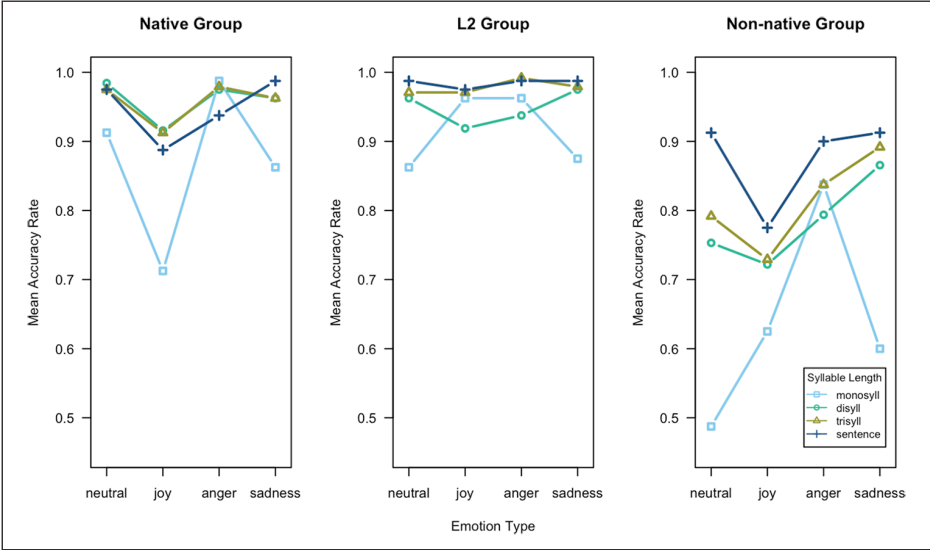
Figure 3. Plots of interaction between emotion type and syllable length for three groups in terms of mean accuracy rate.
